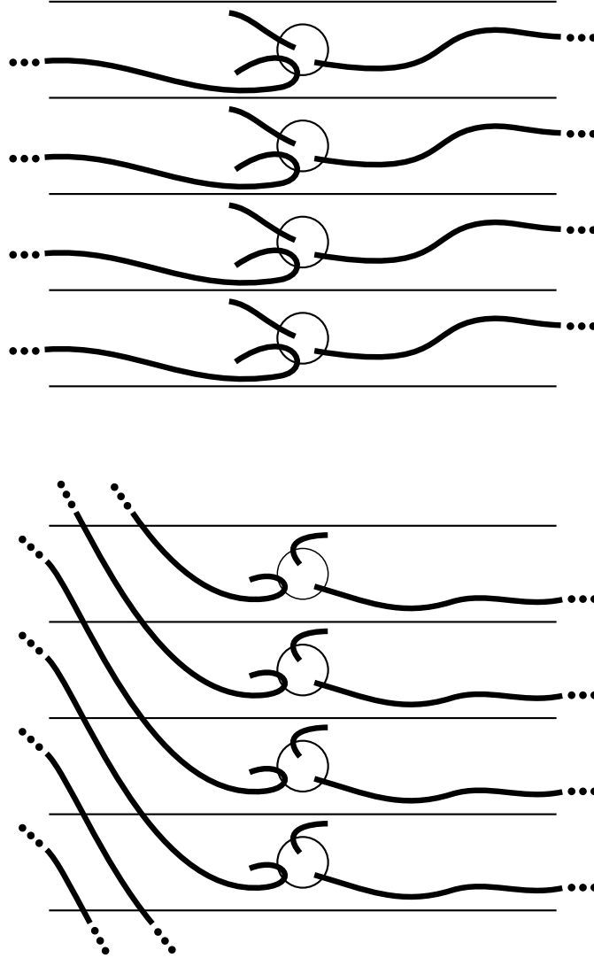
FIGURE 2. An illustration of an example of the set \mathbf{X}^t at t = 0 (above) and at a later moment t > 0 (below). The horizontal lines are the preimages of (0, 1) under \widehat{\text{exp}} , and the balls depicted are the sets \mathbf{E}_n \left( \frac{|\Theta(b^t)|}{2} \right) .
